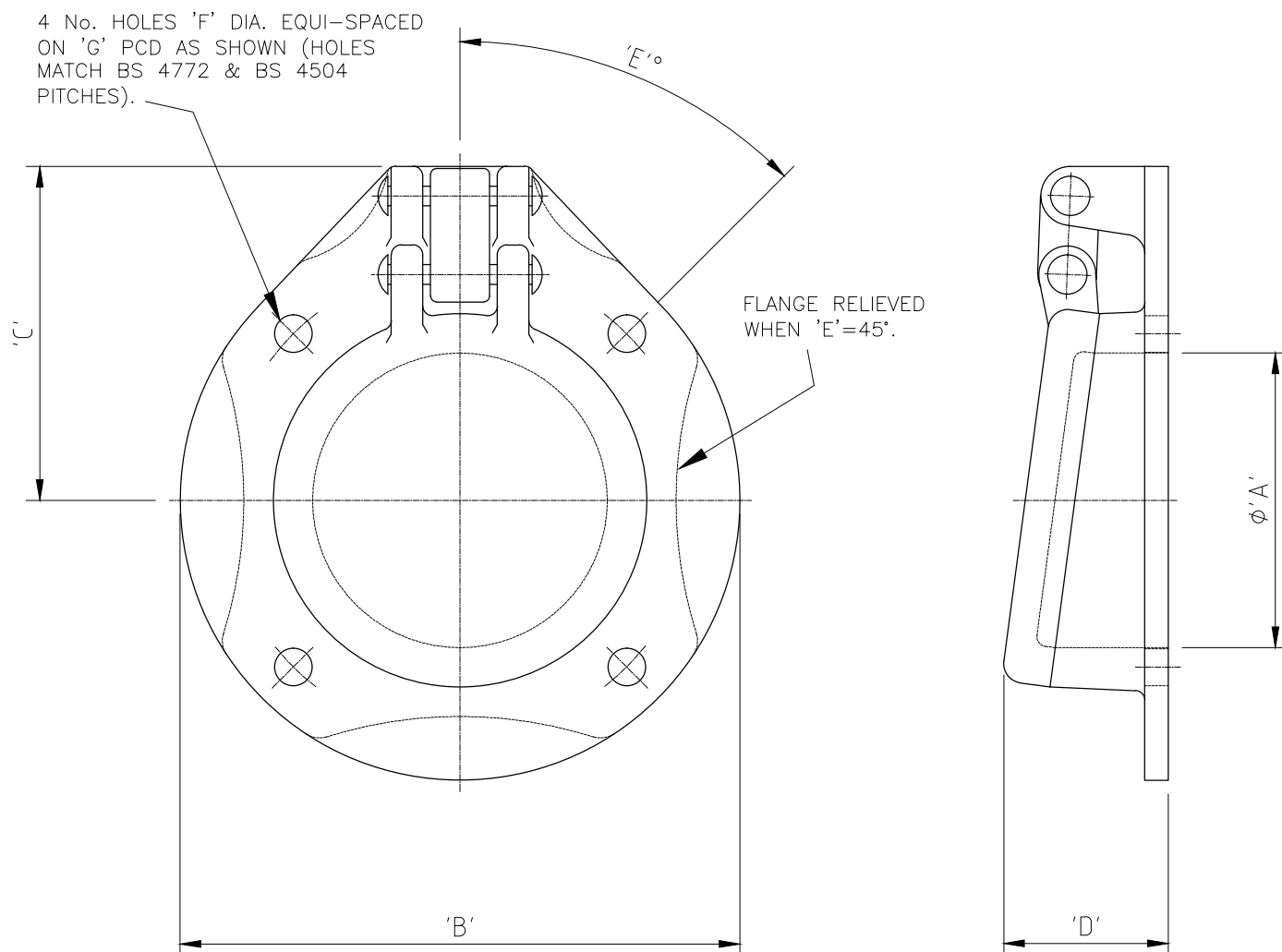
FLAP VALVE DIMENSION TABLE
