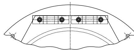
HINGE ARRANGEMENT FOR 400MM SIZES &amp; ABOVE
