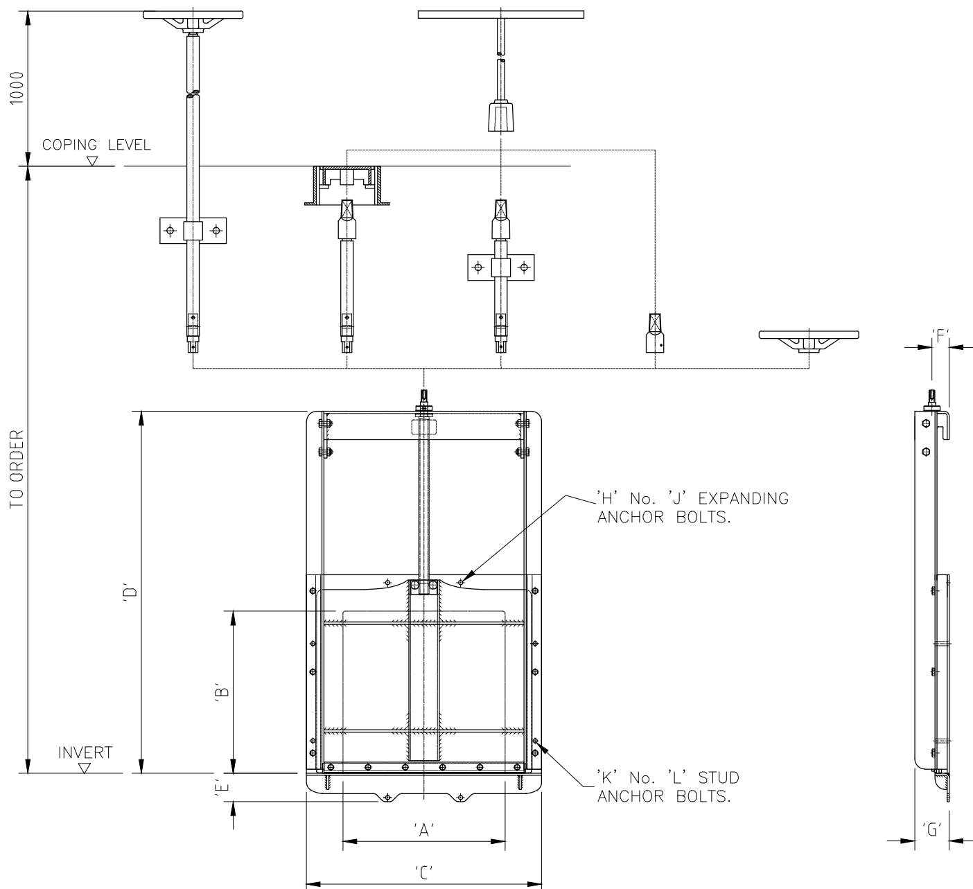
PENSTOCK DIMENSION TABLE
