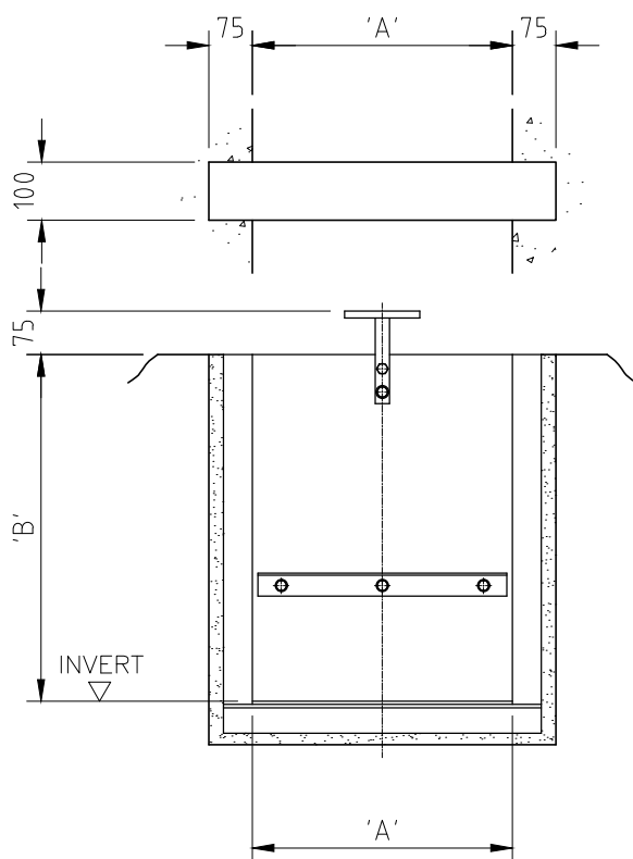
UPTO &amp; INCLUDING 500MM WIDE OPENING
