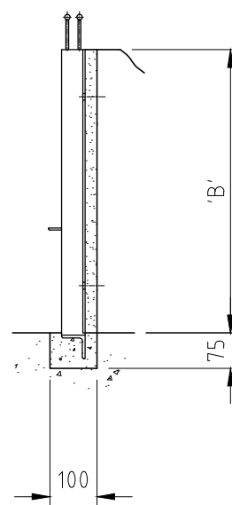
HANDSTOP DIMENSION TABLE
